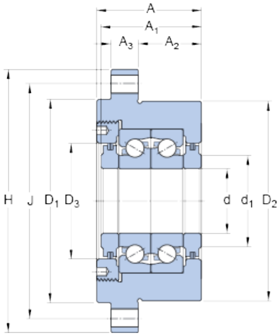
FBSA 210/DF Bearing 2D drawings and 3D CAD models
